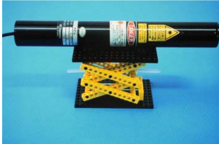
Fig. 7. Laboratory jack carrying a He-Ne laser tube. The approximate weight of the laser is \sim 0.5 Kg.
